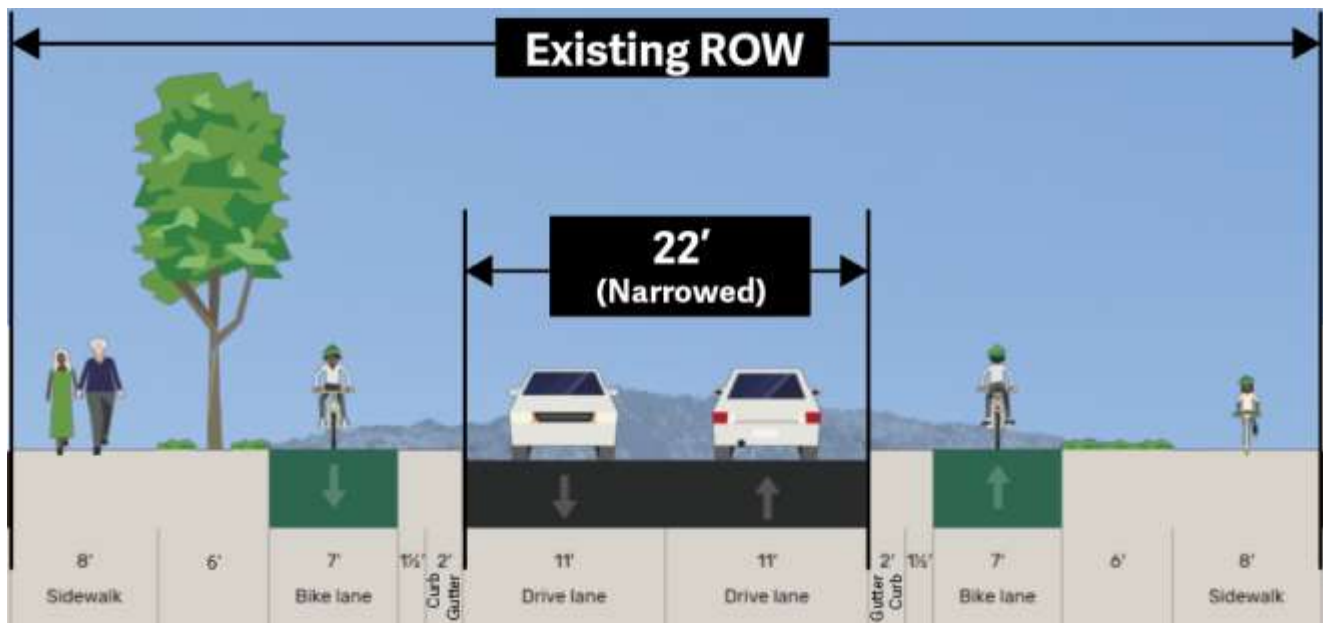
Figure 2: Option 2.1: Two vehicle lanes with off-street protected bike lanes meeting preferred design widths and with improvements behind the curb (Looking West)
