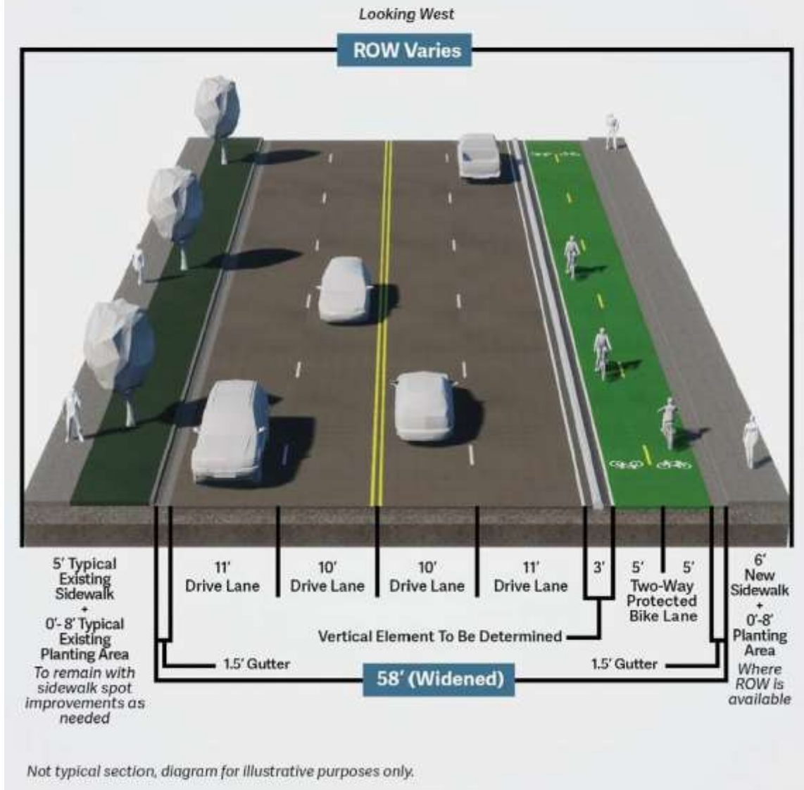
Figure 25: Alternative D: Two-Way Protected Bike Lane and Widened Roadway
